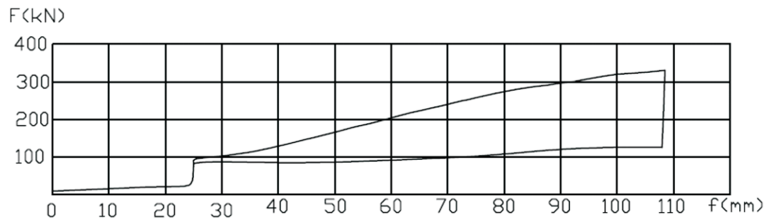
STATIC CHARACTERISTIC
